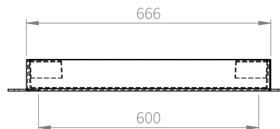
DETAIL B SCALE 1 : 3
